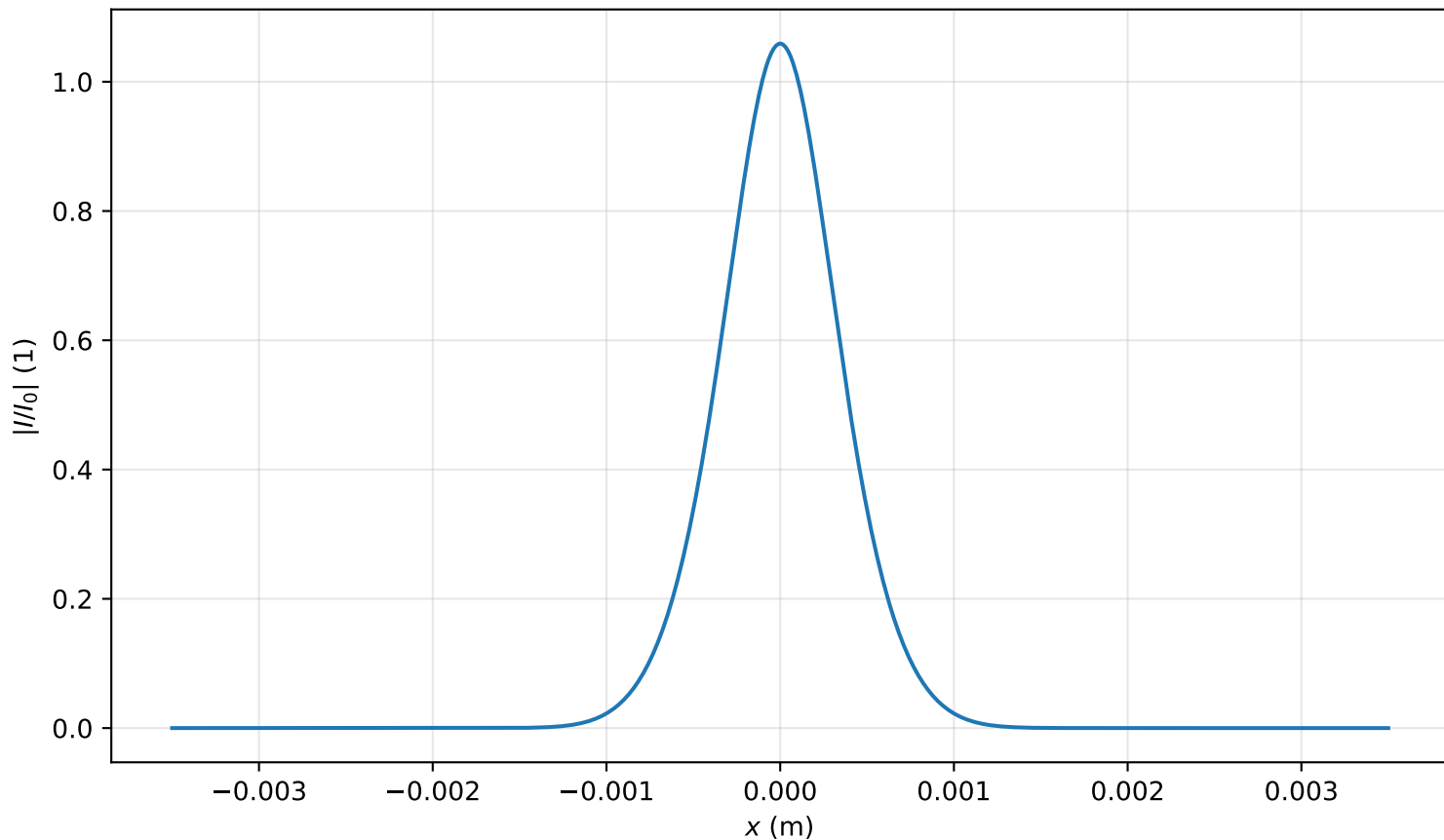
Intensity profile I(x, y = 0, z = 0.716m)/I_0 , P_{in}=0.5P_{cr} , artificial time
